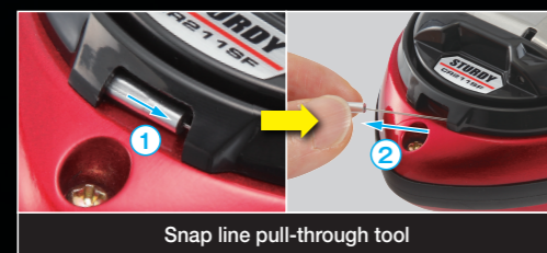
Snap line pull-through tool
