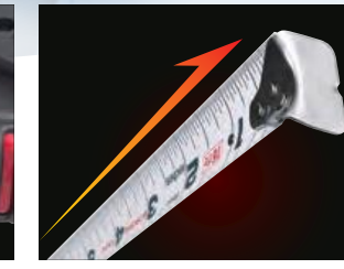
STRONG TAPE & HOOK With a thickness of 1.6 mm, the specially designed Strong Hook has an increased strength of 4.7x more than standard Tajima hooks.
